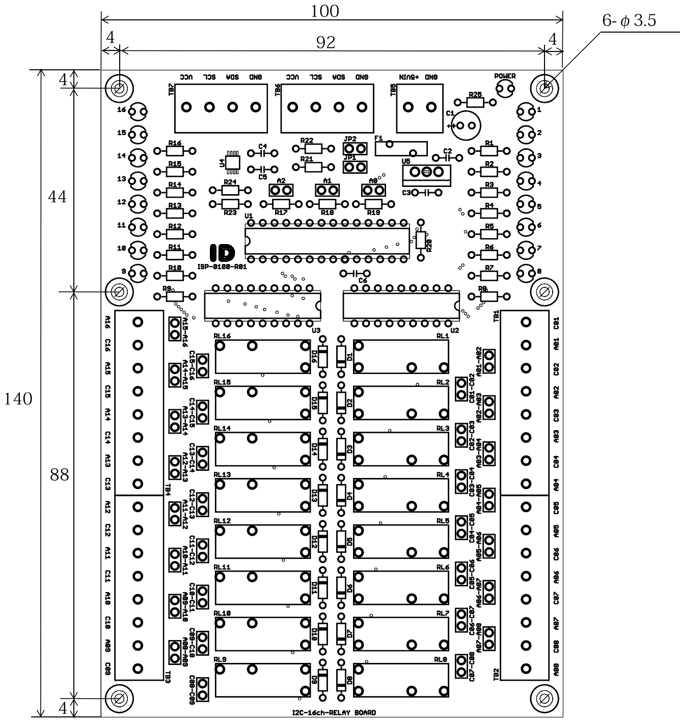
I2C-16ch-RELAY BOARD
